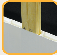
1-3/4" x 32" PVC wall plank is designed to accommodate 2x4 lumber for added strength.
