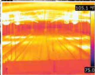
AV Series Heat Distribution - Infrared photos courtesy of Auburn University, National Poultry Technology Center (House pictured is 66' wide)
